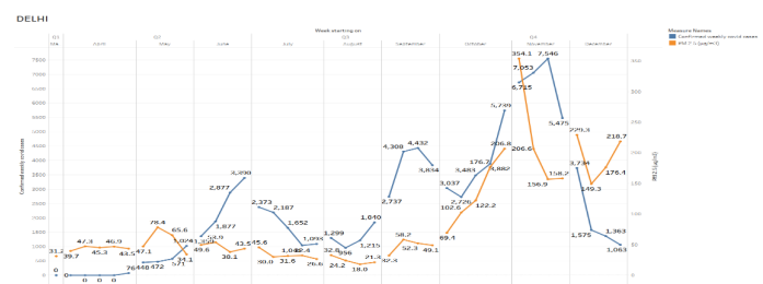
Fig. 5: Covid-19 cases and PM-2.5 in Air of Delhi
