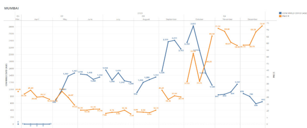
Fig. 6: Covid-19 cases and PM2.5 in Air of Mumbai
