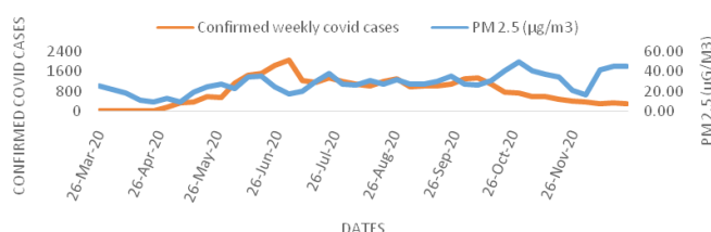
Fig. 8: Covid-19 cases and PM2.5 in Air of Chennai
