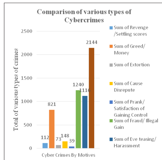
Figure 3. Comparison of various types of Cybercrimes.
