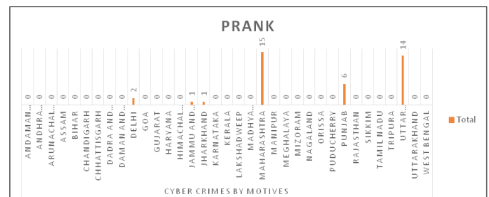
Figure 7. State-wise Analysis of Cybercrime Prank.
