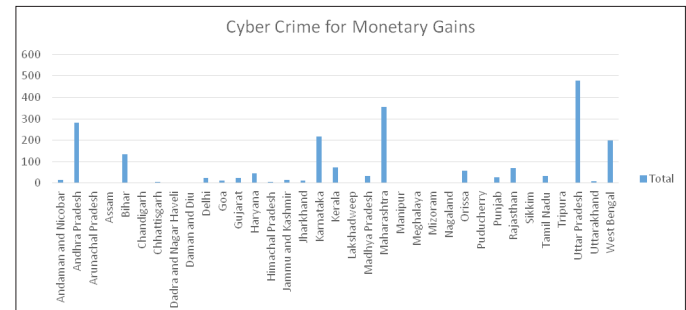
Figure 11. State-wise Analysis of Cybercrime for Monetary Gains.
