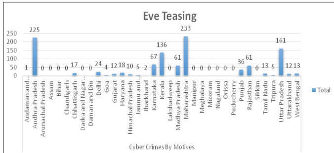
Figure 9. State-wise Analysis of Cybercrime Eve Teasing.
