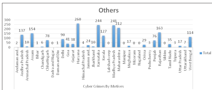
Figure 10. State-wise Analysis of Other Cybercrimes.
