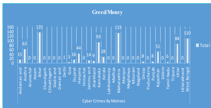
Figure 5. State-wise Analysis of Greed/Settling Score.
