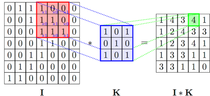
Figure 3. One single operation involving the Kernel (K) and Input (I) at a stage of the convolution to extract features.
