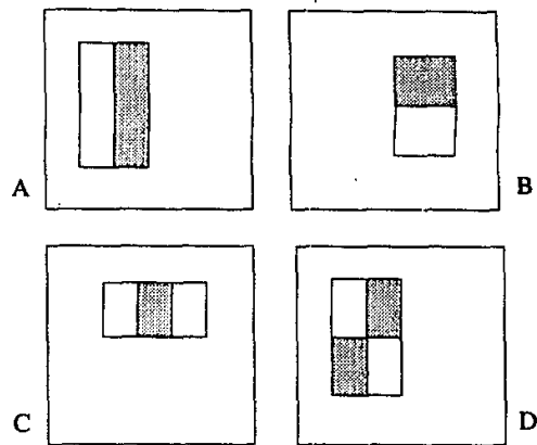
Figure 2. For example, the above squares featuring rectangles show features relative to the detection window. The sum of the pixels which lie within the white rectangles are subtracted from the sum of pixels in the grey rectangles. Nivo-rectangle features are shown in (A) and (B). Figure (1) shows a three-rectangle feature, and (D) a four-rectangle feature 3 .
