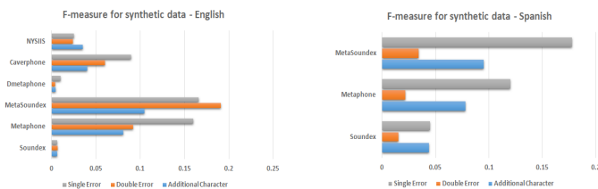
Figure 3. F-measure of different algorithms on synthetic data for English and Spanish languages.
