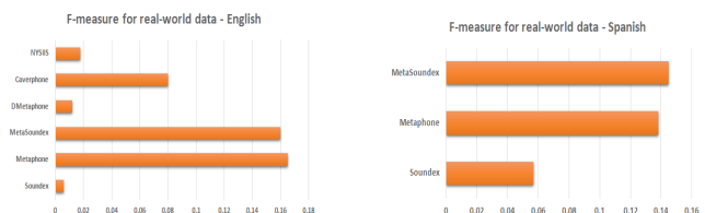
Figure 4. F-measure of different algorithms on real-world misspelled data for English and Spanish languages.
