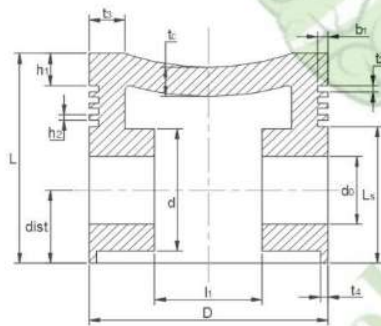
Figure 1. Piston terminology.
